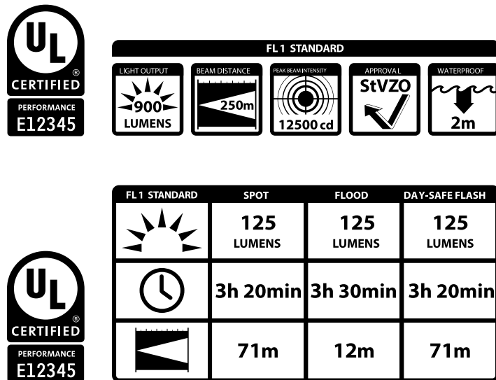
Example icons of ANSI/PLATO FL 1 – 2019 UL S8001 Flashlight Performance
